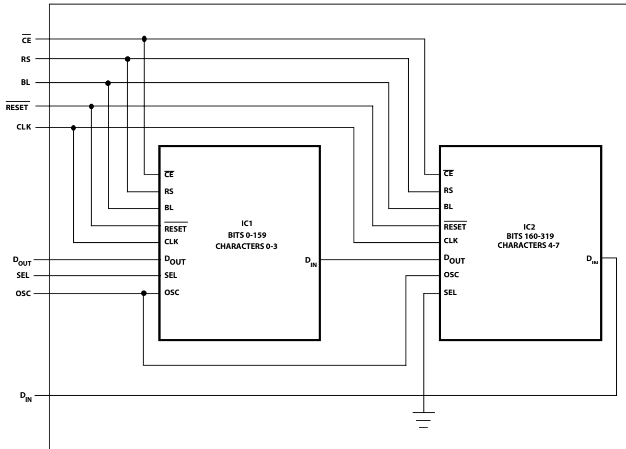
Figure 6. Cascaded ICs.
