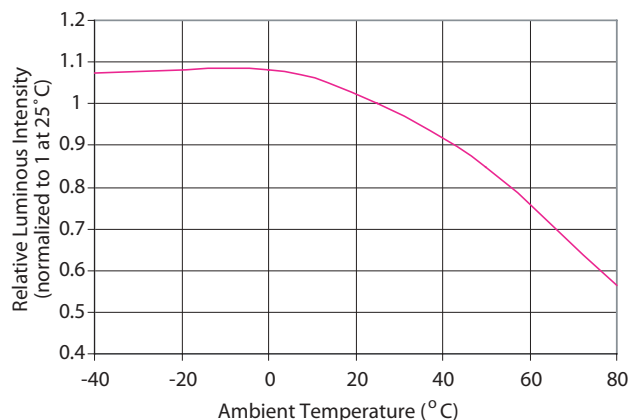
Figure 8. Relative luminous intensity versus ambient temperature.
