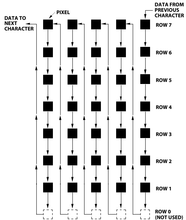
Figure 4. Pixel Map
