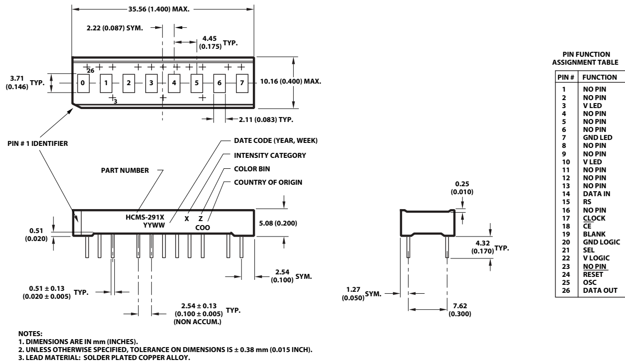
Figure 1. HCMS-2919 package dimension
