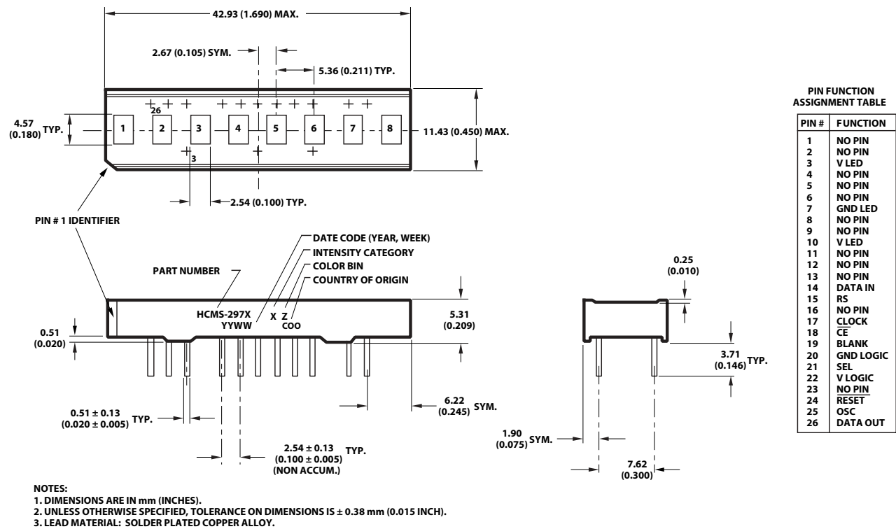
Figure 2. HCMS-2976 package dimensions
