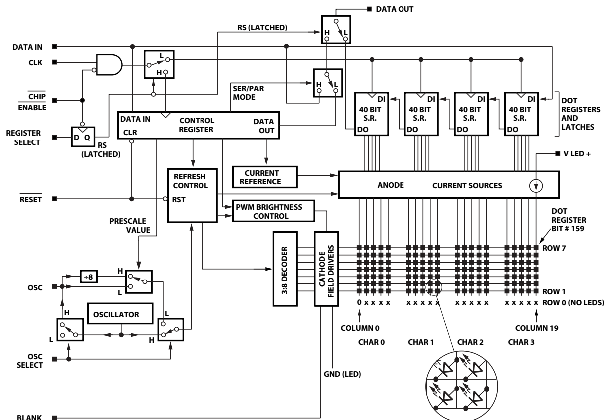
Figure 5. Block diagram
