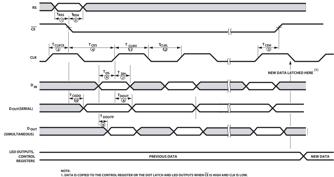
Figure 3. Write Cycle Timing Diagram
